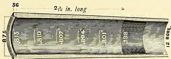
The 12-bore Cartridge Chamber.
